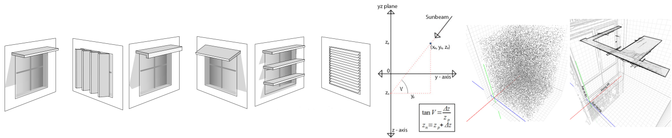
Figure 1: Left: Example typical sun-shades [10] tested for effectiveness comparisons with fittest 10 evolved sun-shades. 3rd-right: Computing sun-ray vector intersection with sun-shades [11]. 2nd-right: Initial 20000 points for evolutionary sun-shade design. Far-right: Example fittest evolved sun-shade for east facing façades in Cape Town (experiment set 1).
